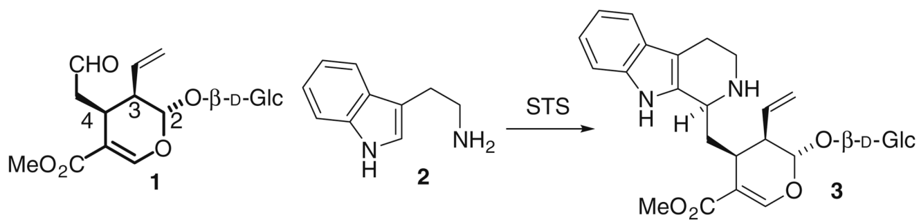
Scheme 1. Pictet-Spengler reaction catalyzed by strictosidine synthase (STS).
